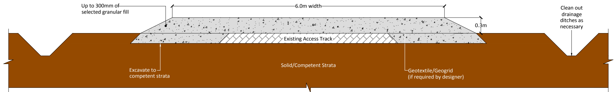
Widening of Access Track on Both Sides
