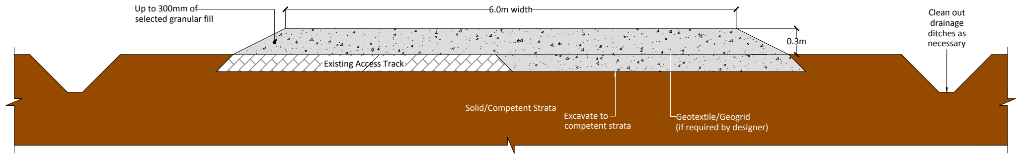
Widening of Access Track on One Side Only
