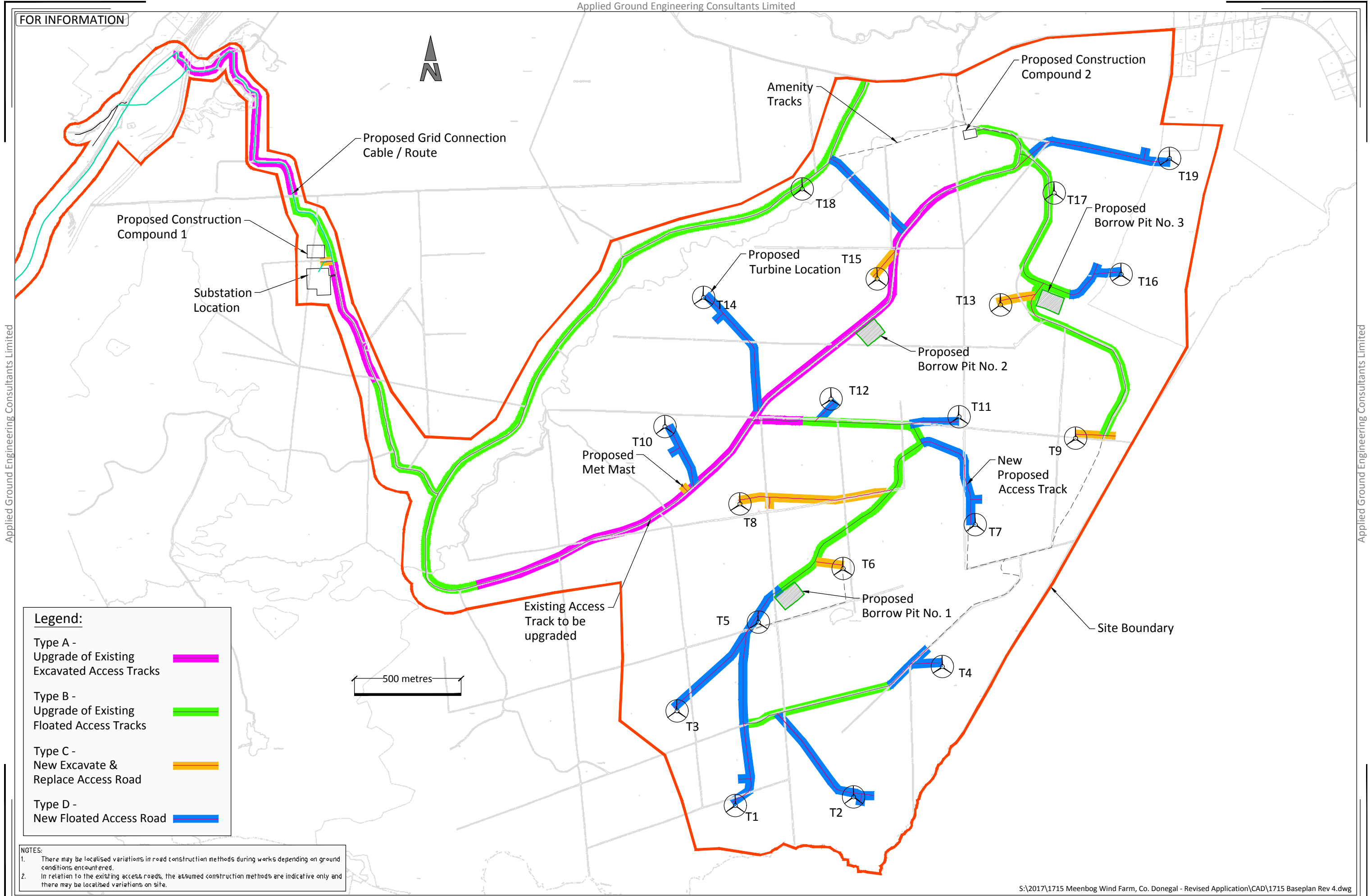
Figure 1 Plan Drawing of Wind Farm with Road Construction Type
